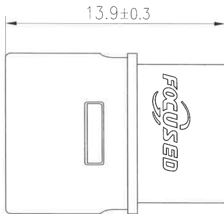
FCB20-F含后盖尺寸
